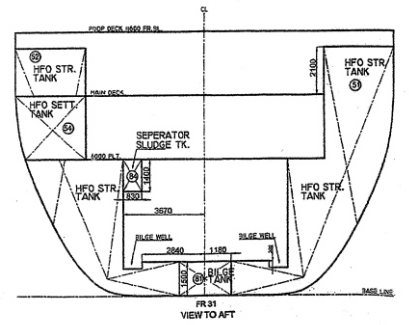
FR 31 VIEW TO AFT
